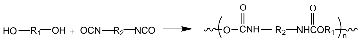
Figure 2 Urethane structure
